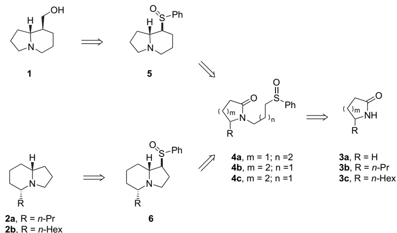
Scheme 1. Retrosynthetic analysis.
